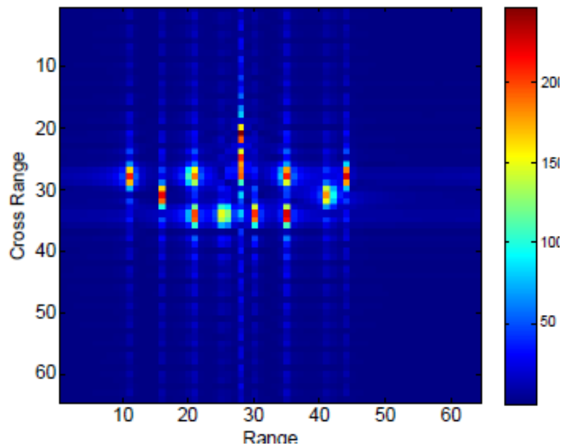
Fig.3. ISAR image using STFT for F=3GHz
